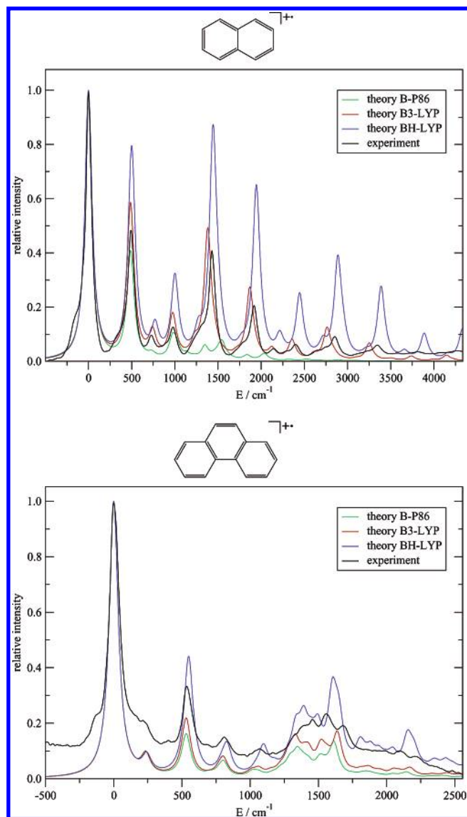
Figure 10. Top panel: Comparison of the calculated and experimental 59 absorption spectra for the 1^2A_u \rightarrow 1^2B_{3g} transition of the naphthalene radical cation ( 34 ). Bottom panel: Comparison of the calculated and experimental 60 absorption spectra for the 1^2B_2 \rightarrow 1^2A_2 transition of the phenanthrene radical cation ( 36 ).
