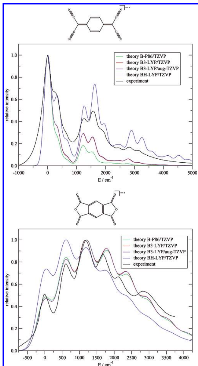
Figure 11. Top panel: Comparison of the calculated and experimental 63 absorption spectra for the 1^2B_{2g} \rightarrow 1^2B_{1u} transition of the radical anion 38 . Bottom panel: Comparison of the calculated and experimental 64 absorption spectra for the 1^2A_u \rightarrow 1^2B_{2g} transition of the radical anion 39 .
